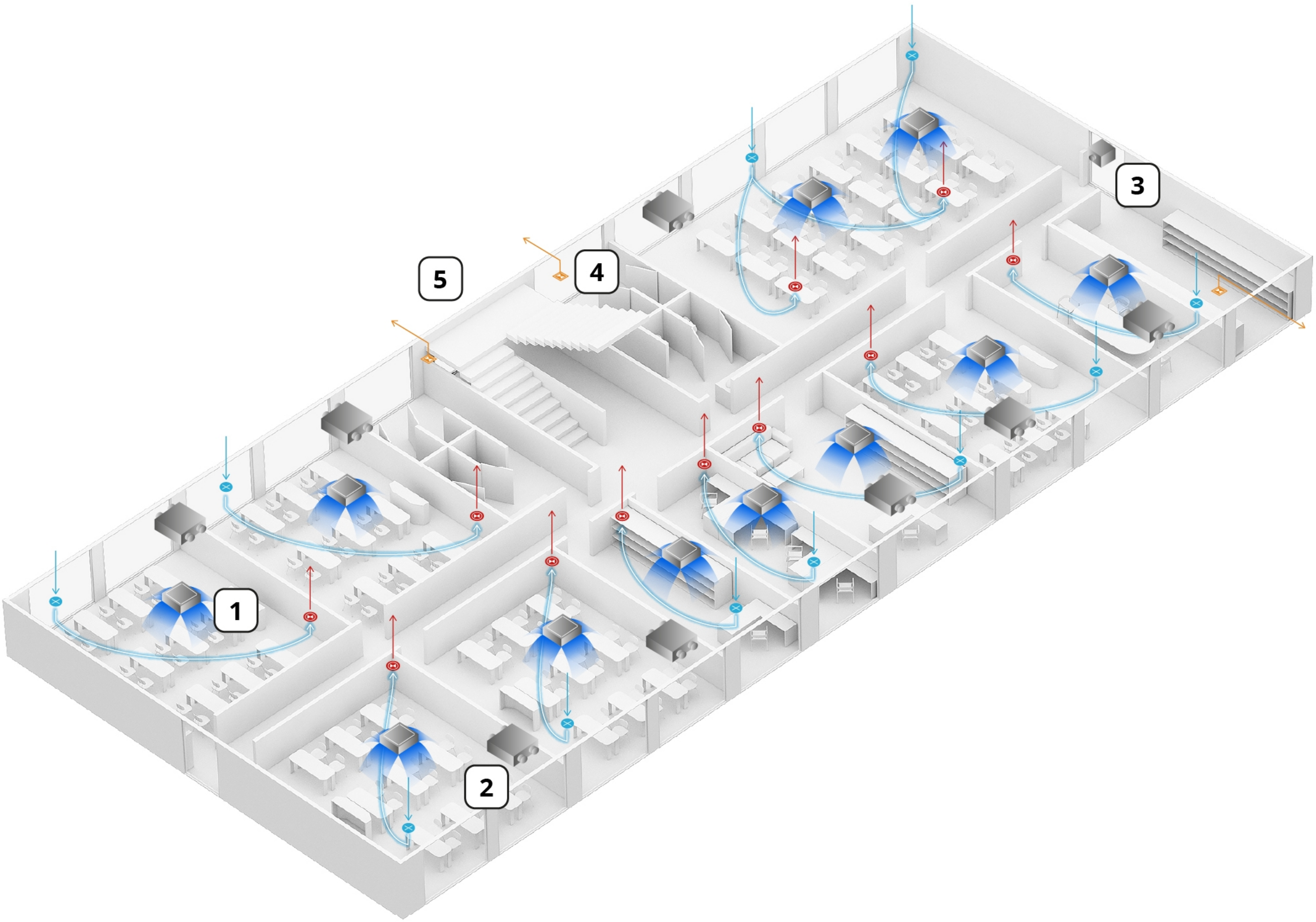
4-way cassette
