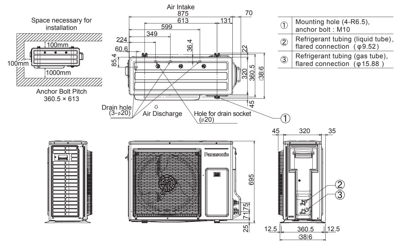
Dimensions (U-30PN1H5) 1-phase (U-30PN1H8 / U-36PN1H8) 3-phase
