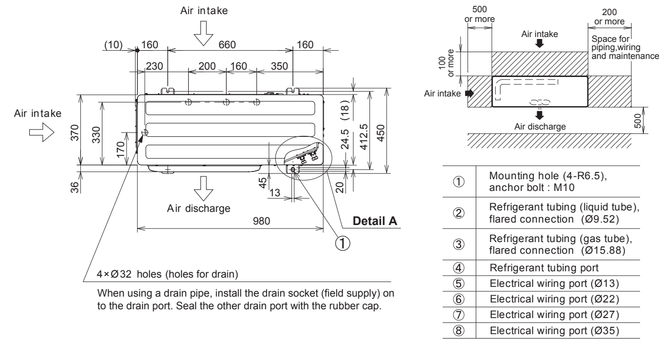
Dimensions (U-42PN1H8 / U-50PN1H8) 3-phase
