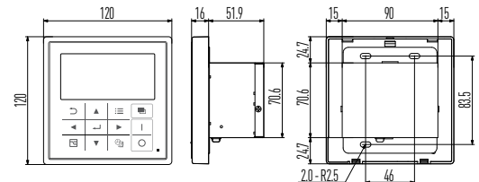
SYSTEM CONTROLLER (CZ-64ESMC3)
