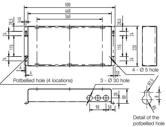
LONWORKS INTERFACE (CZ-CLNC2)
