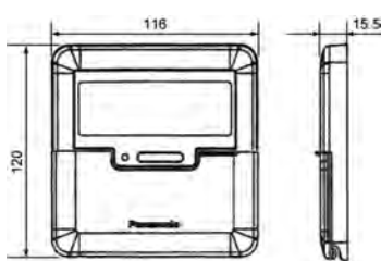
WIRED REMOTE CONTROLLER FOR RESIDENTIAL MODEL (CZ-RD52CP)
