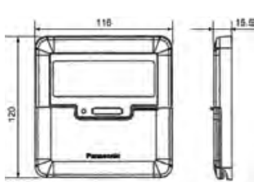
WIRED REMOTE CONTROLLER FOR RESIDENTIAL MODEL (CZ-RD52CP)
