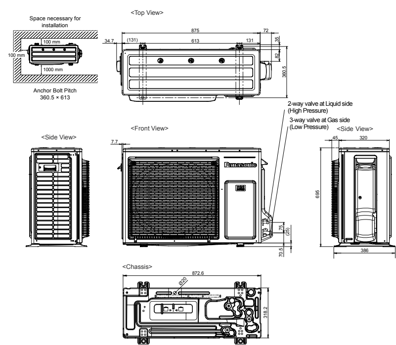
Dimensions (4.8kW – 5.7kW) CU-Z50UBRA / CU-Z60UBRA
