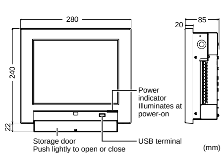
INTELLIGENT CONTROLLER (CZ-256ESMC3)
