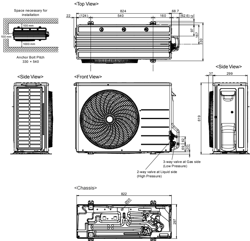
Dimensions (3.5kW – 3.7kW) CU-Z35UBRA
