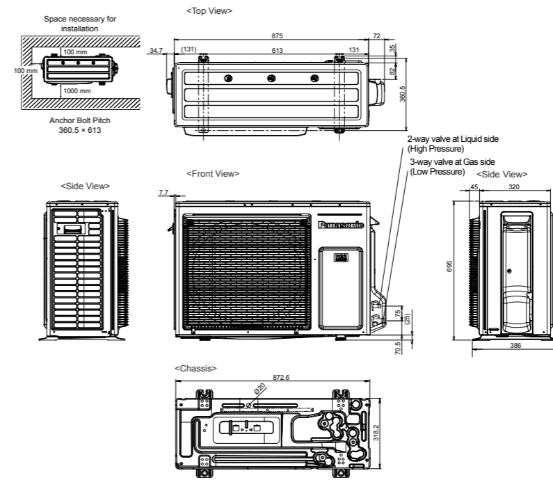
Dimensions (4.8kW – 5.7kW) CU-Z50UBRA / CU-Z60UBRA
