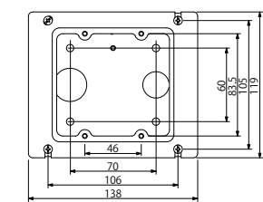
Switch box
