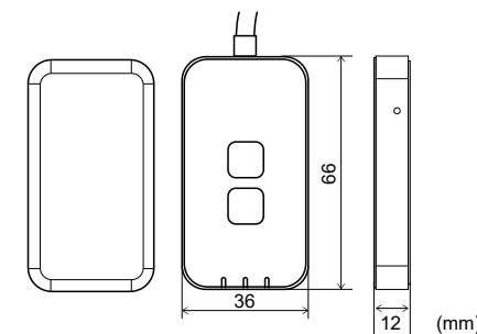
WLAN ADAPTOR (CZ-TACG1)
