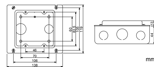
Switch Box
