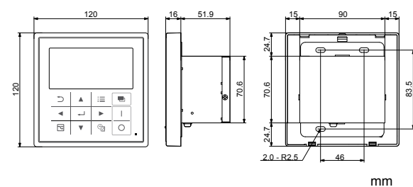
System Controller
