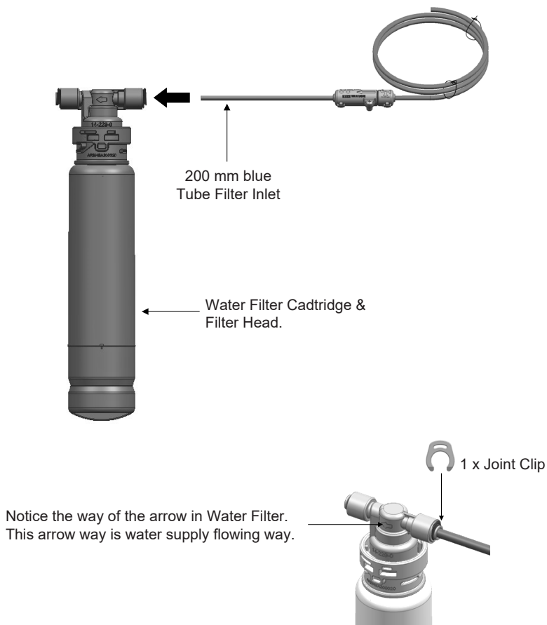
Figure 1: Connect 200 mm Tube Filter Inlet of Dual Check Valve Assembly Block with Water Filter Cartridge & Filter Head
