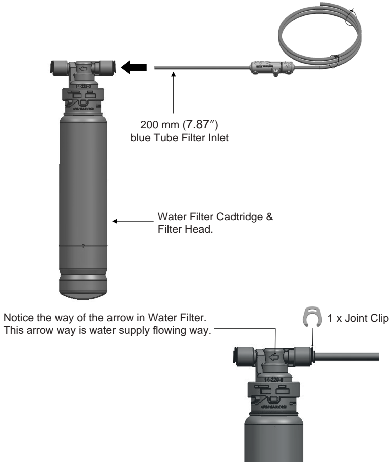
Figure 1: Connect 200 mm (7.87") Tube Filter Inlet of Dual Check Valve Assembly Block with Water Filter Cartridge & Filter Head
