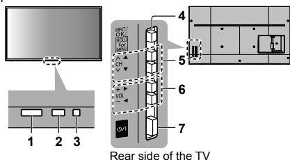
Rear side of the TV
