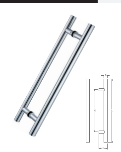
Handle LS-Y02 Series
