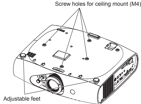
The positions of screw holes for ceiling mount and adjustable feet
