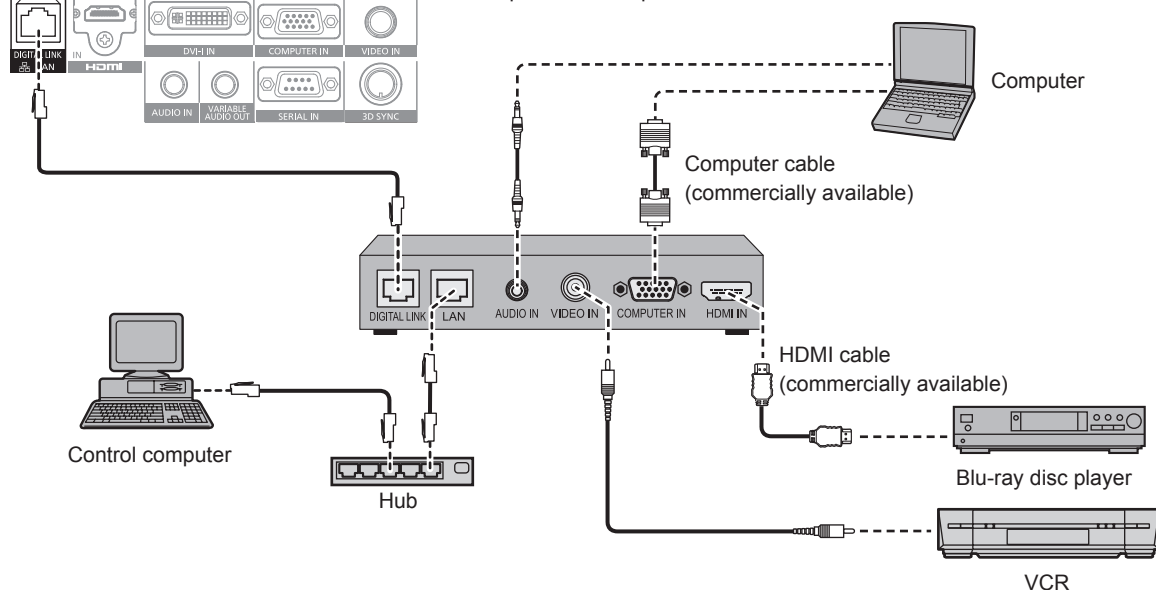
Example of twisted-pair-cable transmitter
