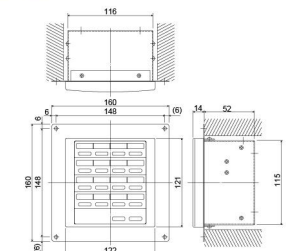
LonWorks介面CZ-CLNC2
