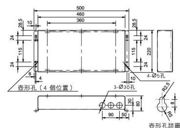
LonWorks介面CZ-CLNC2
