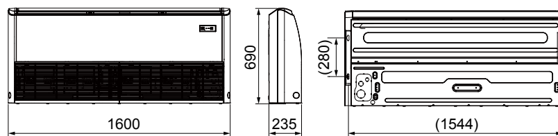
48,000 - 60,000 Btu/h
